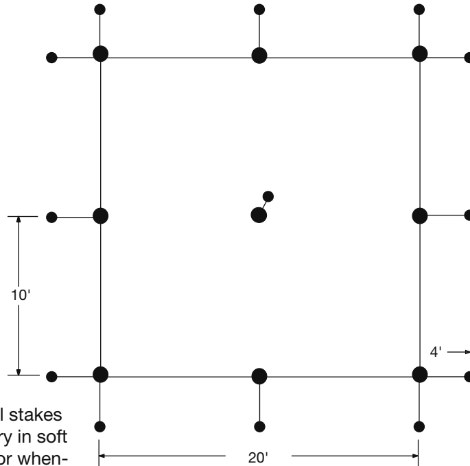
PLAN W/STAKES
